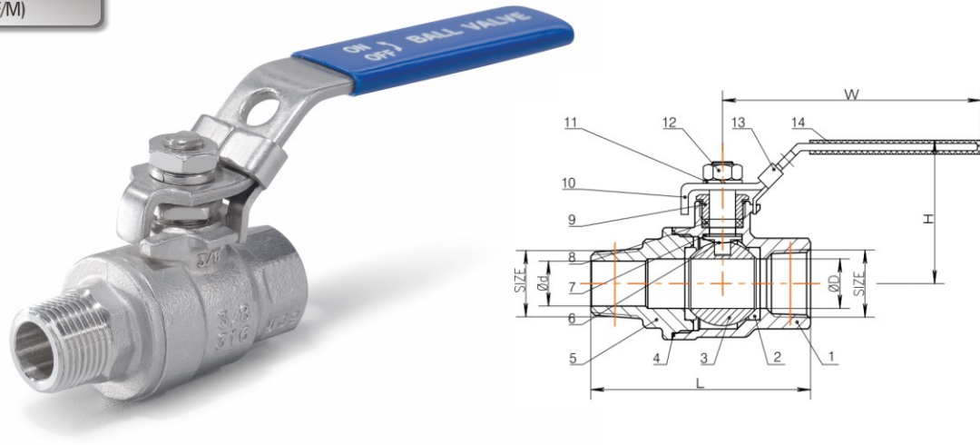
422 Series 2-PC Ball Valve (F/M)
