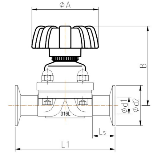
Tri-clamp connection
