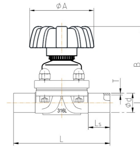
Welded connection
